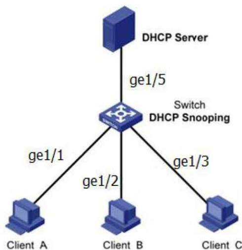
Configure DHCP snooping to support Option 82
